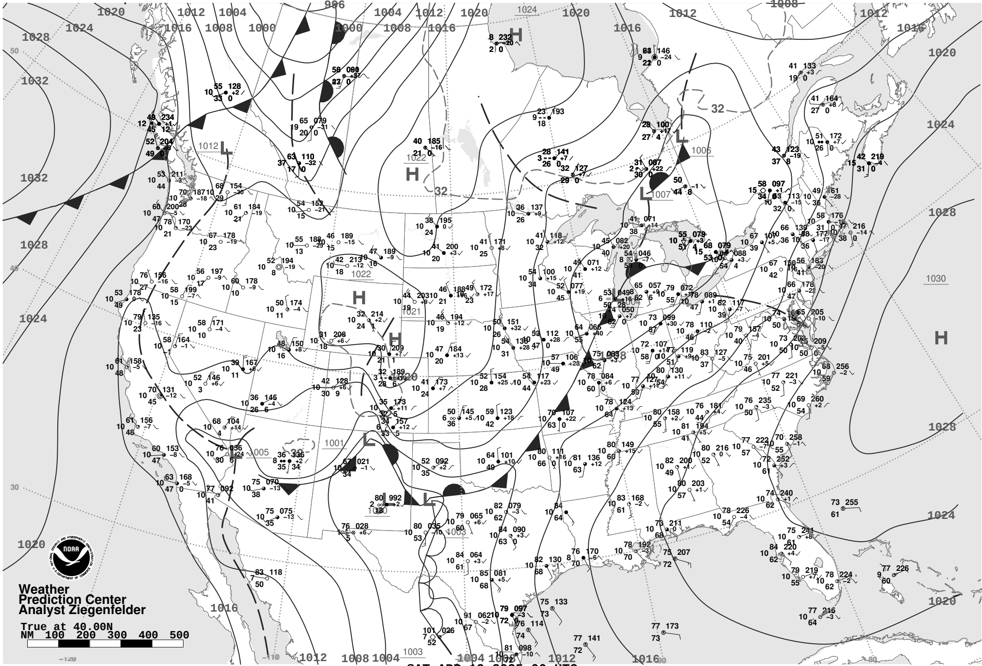
SAT APR 19 2025 00 UTC Surface Weather Map and Station Weather
