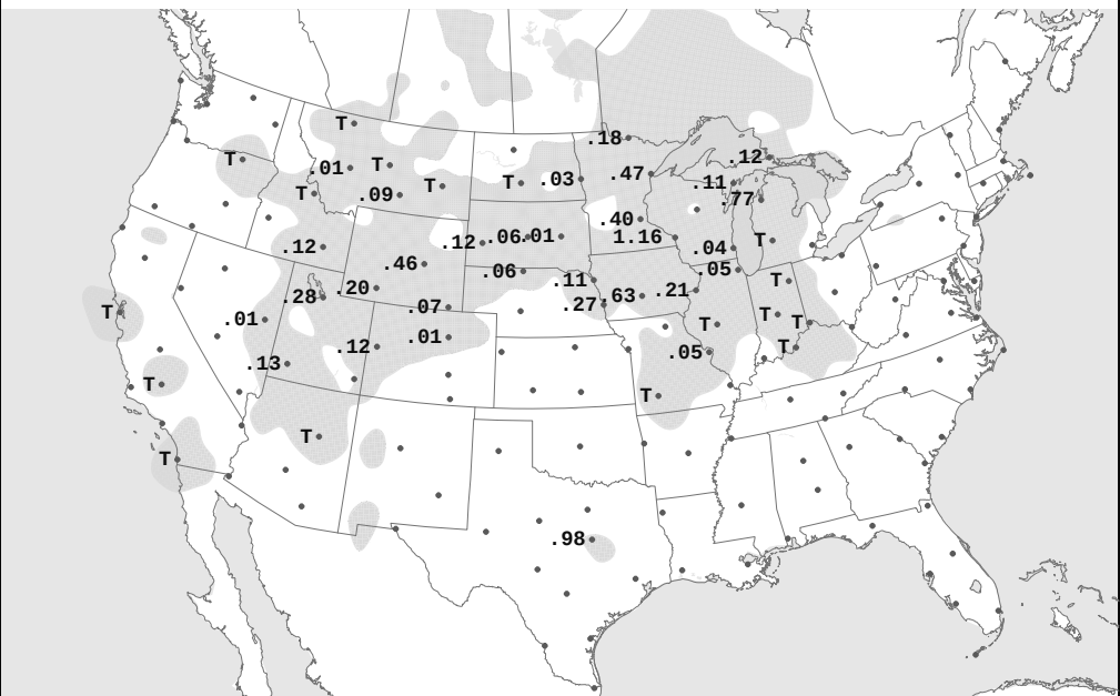
FRI, APR 18, 2025 24-hour Precipitation Areas and Amounts Ending 7:00 A.M. E.S.T.
