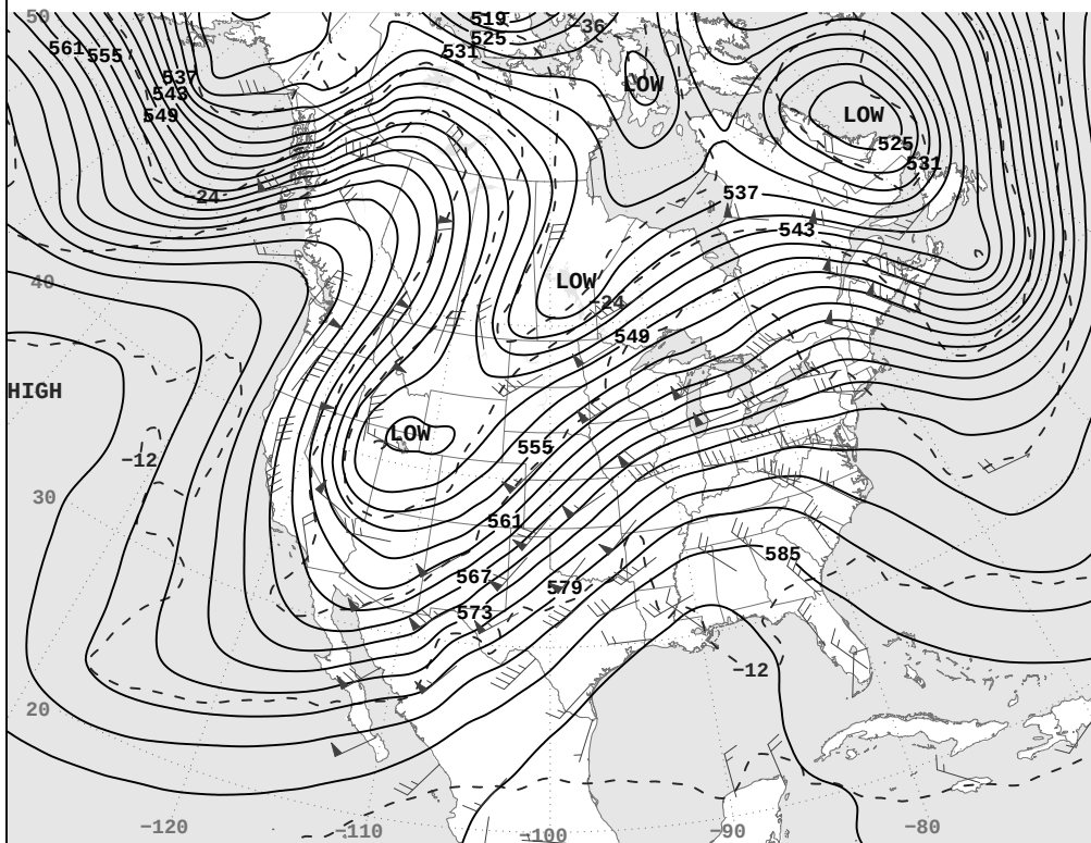
FRI, APR 18, 2025 500-Millibar Height Contours at 7:00 A.M. E.S.T.
